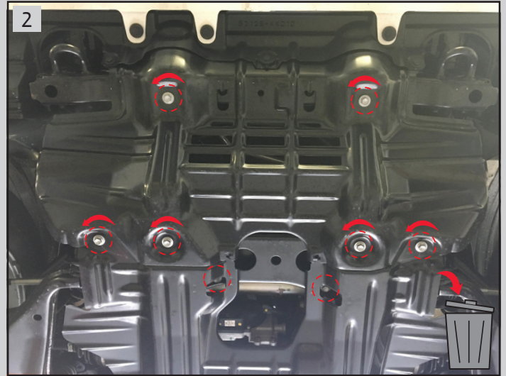
Remove 8 bolts and dispose the original plate
