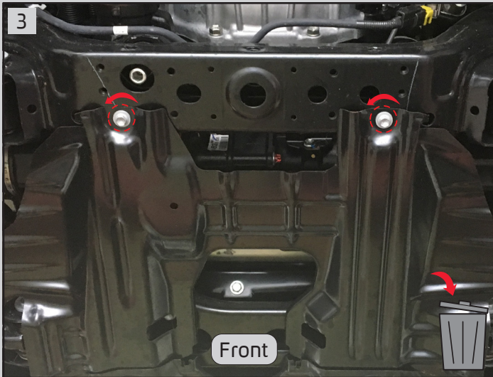
Remove 2 bolts and dispose the original plate
