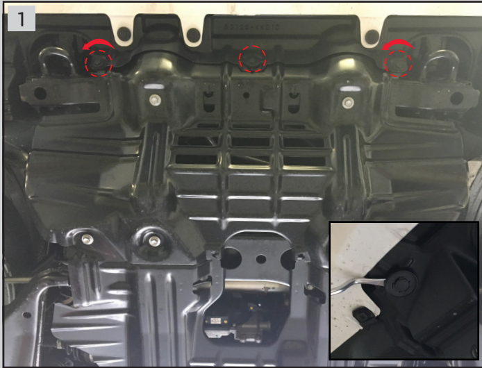
Remove 2 bolts and the middle clip
